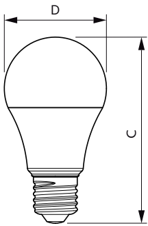
Bulb A60 HV 11-W 1250lm 6500K E27 ND FR
